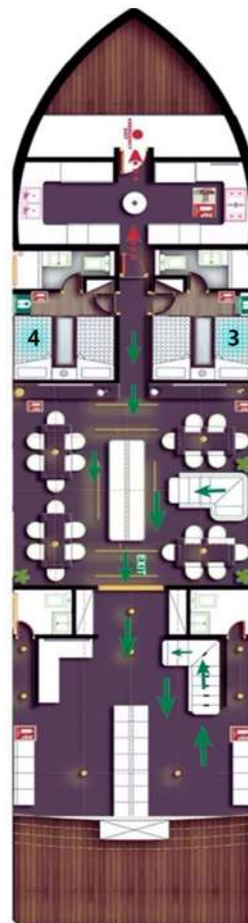
#MAIN DECK
