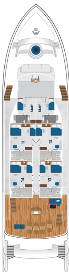
#UPPER DECK
